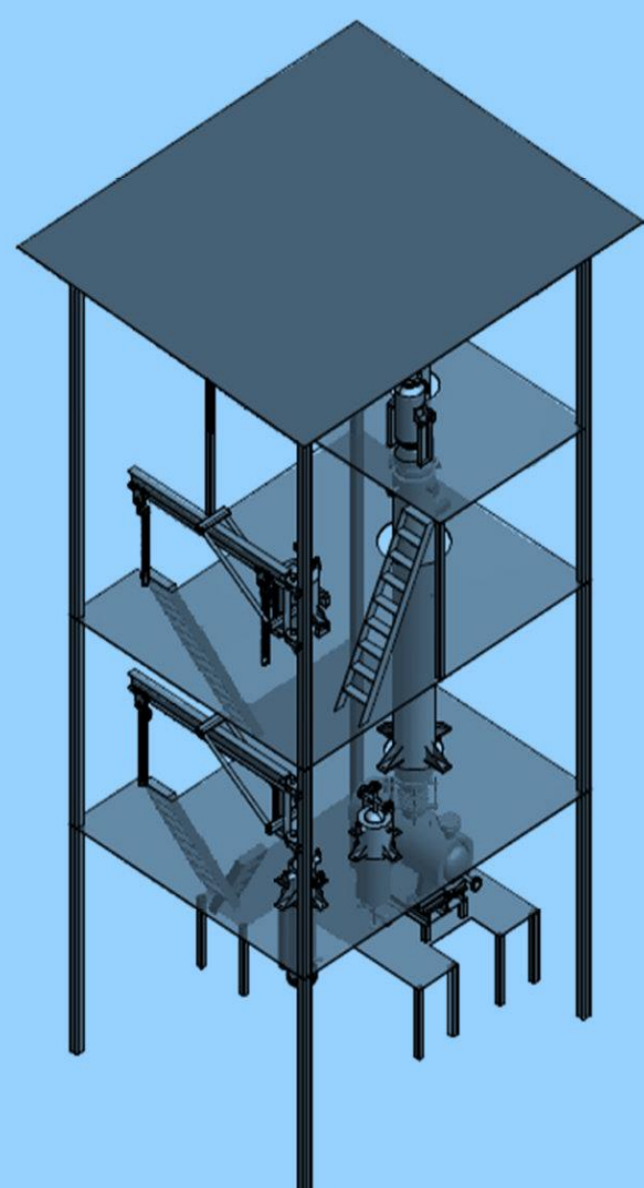
Batch Distillation Plant - Somersby
